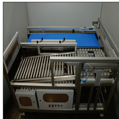
ROLLER CONVEYOR
