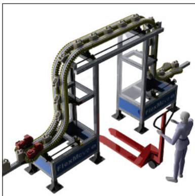
WEDGE CONVEYOR
